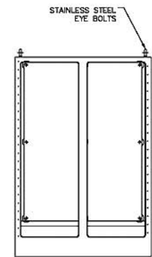
FRONT VIEW WITH DOORS REMOVED
